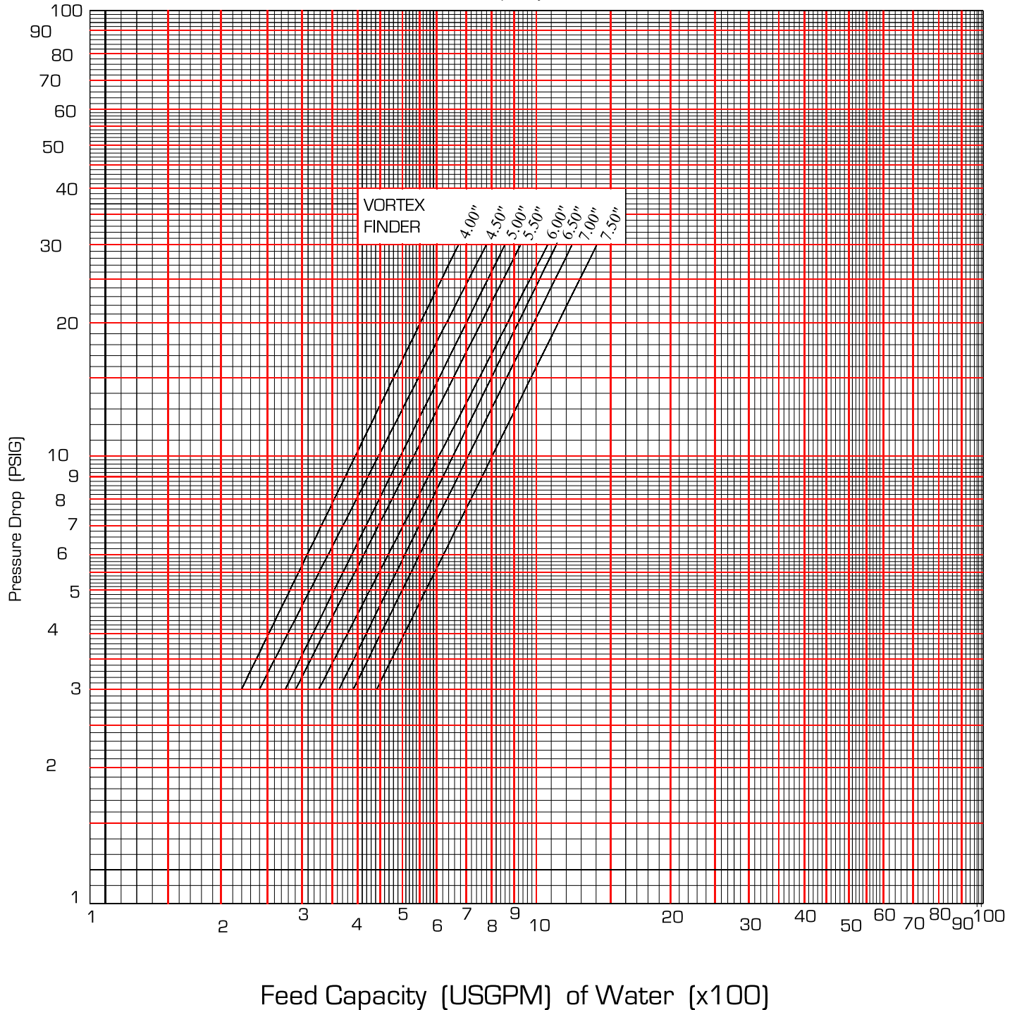
Capacity Curve
